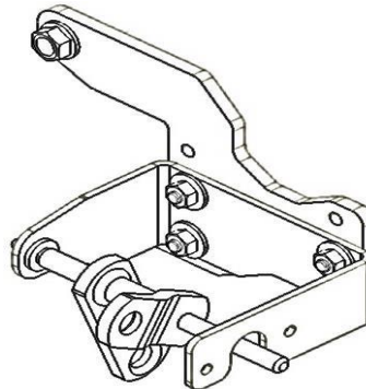
Figure 6 Transfer Case Linkage
